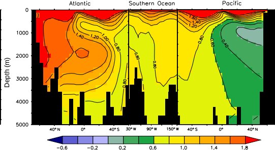
(b) \delta^{13}\text{C} (‰) Bern3D model
