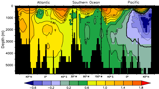
(a) \delta^{13}\text{C} (‰) Eide et al., 2017
